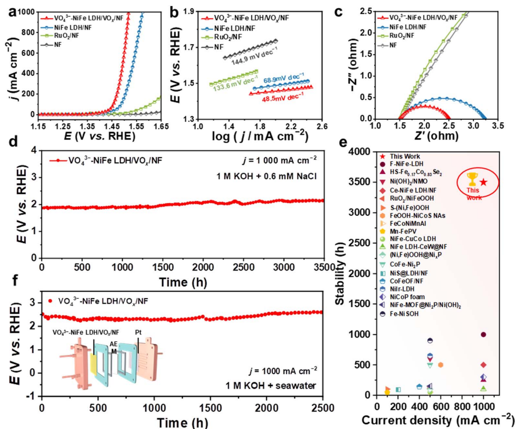
Fig. 2 (a) OER polarization curves of all catalysts in 1.0 M KOH + 0.6 M NaCl; (b) Tafel plots; (c) EIS Scheme; (d) durability evaluation by the chronopotentiometry at 1000 mA cm -2 ; (e) comparison of stability with other works; (f) durability evaluation using electrolysis membrane electrode assembly.
