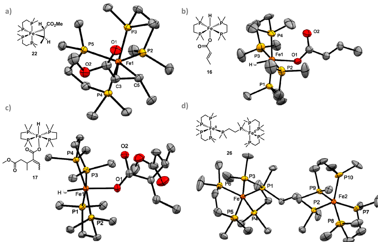
Fig. 4 ORTEP plots of (a) [(dmpe)_2Fe(\eta^2-1)] 22 . (b) Trans - [(dmpe)_2FeH(CH_3CH=CH-COO^-)] 16 . (c) Trans - [(dmpe)_2FeH(CH_3O_2CC_6H_{10}COO^-)] 17 . (d) [(dmpe)_5Fe_2] 26 . Iron, carbon, phosphorus, oxygen and hydride atoms on the molecular structures are coloured orange, grey, yellow, red and white respectively. Hydrogens have been omitted for clarity and thermal ellipsoids have been set at 50% probability.
