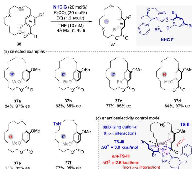
Fig. 9 NHC-catalyzed intramolecular macrocyclization for the synthesis of planar chiral paracyclophanes (Zhao's work).
