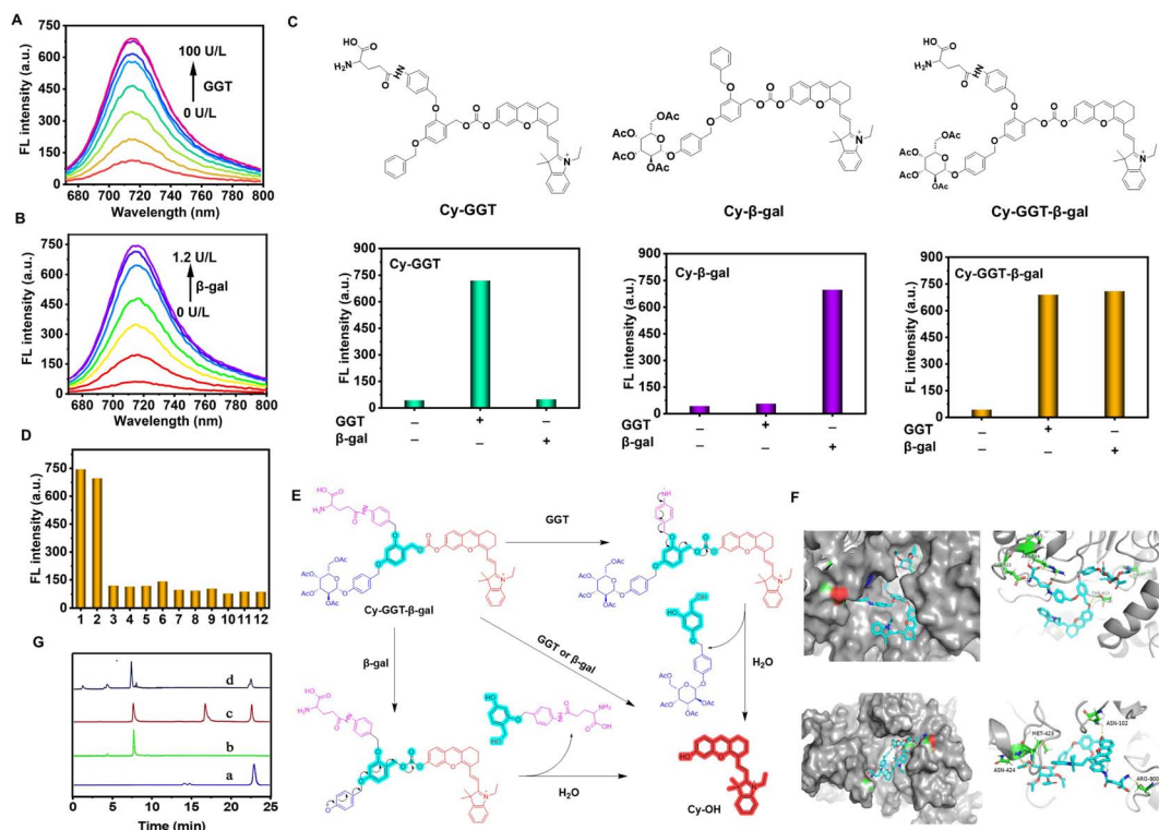
Fig. 1 The fluorescence spectrum changes of Cy-GGT-β-gal ( 5 \mu\text{M} ) in PBS buffer ( 10.0 \text{ mM} , \text{pH } 7.4 , containing 20\% \text{ DMSO} ), after introduction of (A) GGT ( 0.0 – 100.0 \text{ U L}^{-1} ) and (B) \beta -gal ( 0.0 – 1.2 \text{ U L}^{-1} ). (C) The chemical structure of probes Cy-GGT , Cy-β-gal and Cy-GGT-β-gal and the fluorescence intensity of Cy-GGT , Cy-β-gal and Cy-GGT-β-gal ( 5 \mu\text{M} in PBS, \text{pH} = 7.4 , 20\% \text{ DMSO} ) at 2 \text{ h} under different stimuli (GGT, 100 \text{ U L}^{-1} ; \beta -gal, 1.2 \text{ U L}^{-1} ). The above assays were performed at 37 \text{ }^\circ\text{C} without further modification. (D) The fluorescence intensity of Cy-GGT-β-gal ( 5 \mu\text{M} ) at 720 \text{ nm} in various biological species (1. GGT; 2. \beta -gal; 3. NADH; 4. NTR; 5. APN; 6. ALP; 7. BSA; 8. GSH; 9. \text{H}_2\text{O}_2 ; 10. Hcy; 11. Cys; 12. PBS). (E) Proposed mechanism for the reaction between Cy-GGT-β-gal and GGT or Cy-GGT-β-gal and \beta -gal. (F) Molecular docking analysis of Cy-GGT-β-gal interactions: stereoscopic images showing Cy-GGT-β-gal (blue) docked with GGT (grey, upper left) and \beta -gal (grey, lower left) using the flexible docking module in Discovery Studio, with corresponding LigPlot schematic diagrams illustrating the secondary structure interactions (upper and lower right, respectively). (G) HPLC chromatographic analysis was performed on several samples: pure Cy-GGT-β-gal (a), CyI-OH (b), a mixture of Cy-GGT-β-gal with GGT (c) and a mixture of Cy-GGT-β-gal with \beta -gal. Detection was carried out at 670 \text{ nm} for lanes (a–d). The reaction mixture, consisting of ACN/water ( 60 : 40 ) and \text{NaHCO}_3 ( 5 \text{ equiv.} ), was analyzed after a 2 -hour incubation period.
