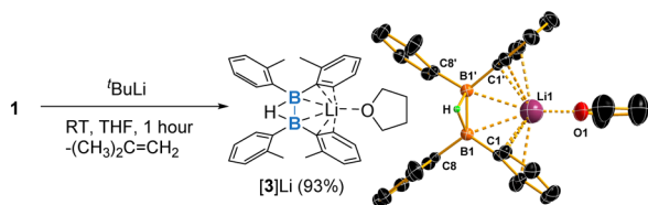
Fig. 2 Reaction of 1 with t\text{BuLi} and the molecular structure of [3]Li (all hydrogen atoms are omitted for clarity except for the bridging H atom). Selected bond distance (Å) and angles (deg.): B–B' = 1.642(6); C1–B1–B1' = 123.98(14); C8–B1–B1' = 120.97(14); C1–B1–C8 = 115.0(2).
