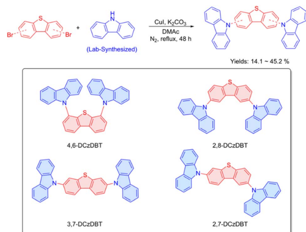
Scheme 2 Synthetic route and chemical structures of investigated ternary \pi -conjugated molecules.
