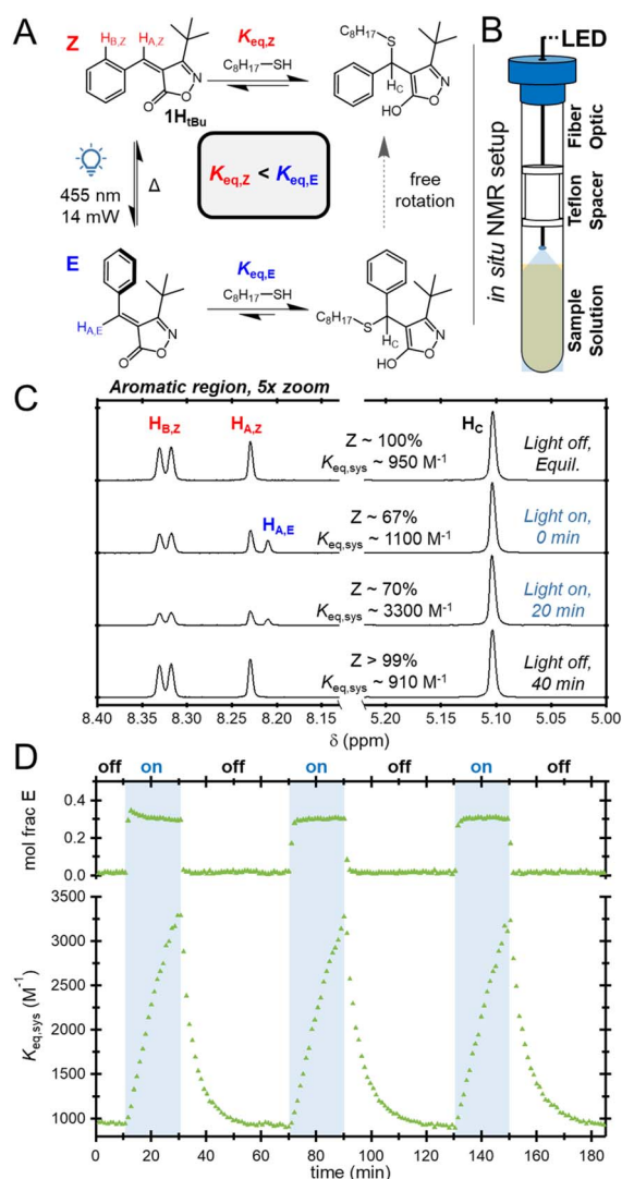
Fig. 3 (A) Equilibria involved in thiol-bonding and photoisomerization. (B) Diagram of the in situ LED NMR setup. (C) ^1\text{H} NMR spectra of 1H t Bu equilibrated with OT without and during irradiation with 455 nm light. (D) Cycling experiment (455 nm irradiation for 20 min followed by a 40 min dark interval) for 1H t Bu equilibrated with OT .
