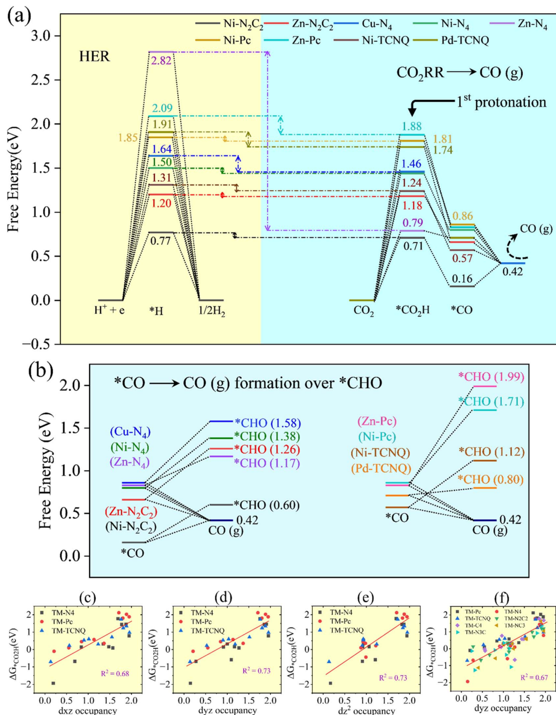
Fig. 2 (a) and (b) the comparison of CO 2 RR and HER selectivity and CO(g) formation over CHO with the nine best SACs; (c)–(e) the correlation of occupancies of d xz , d yz and d z 2 orbitals with the free energy of the first protonation step in the CO 2 → CO(g) pathway for SACs with TMs coordinated with four N-atoms and (f) correlation of the occupancy of d yz with the free energy of the first protonation step in the CO 2 → CO(g) pathway with all 77 SACs.
