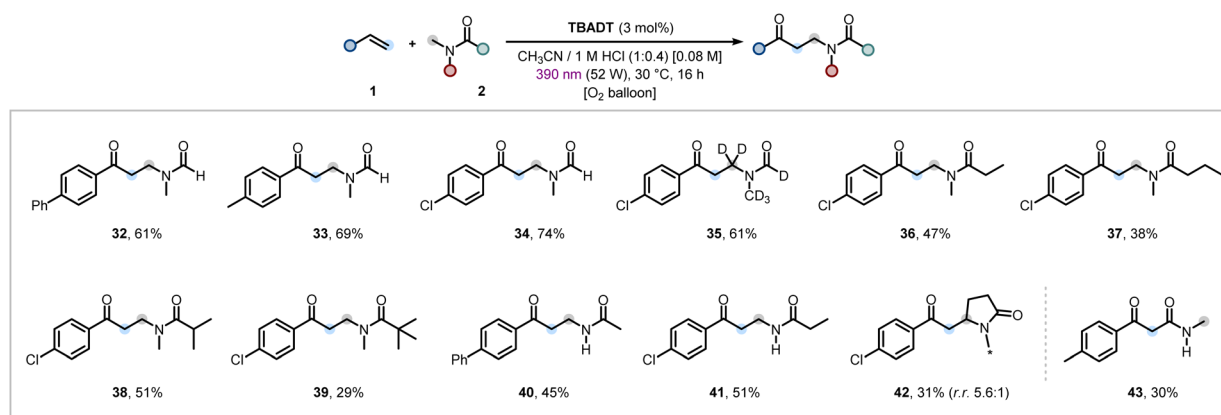
Fig. 3 Scope of the alkene oxo-amidomethylation varying amide partner. Reaction conditions: styrene 1 (0.3 mmol, 1.0 equiv.), amide 2 (1.5 mL, 1.5 equiv.), TBADT (3 mol%), 1 M aqueous HCl (0.6 mL) in anhydrous CH 3 CN (1.5 mL). For further details, see the SI. Isolated yields are reported.
