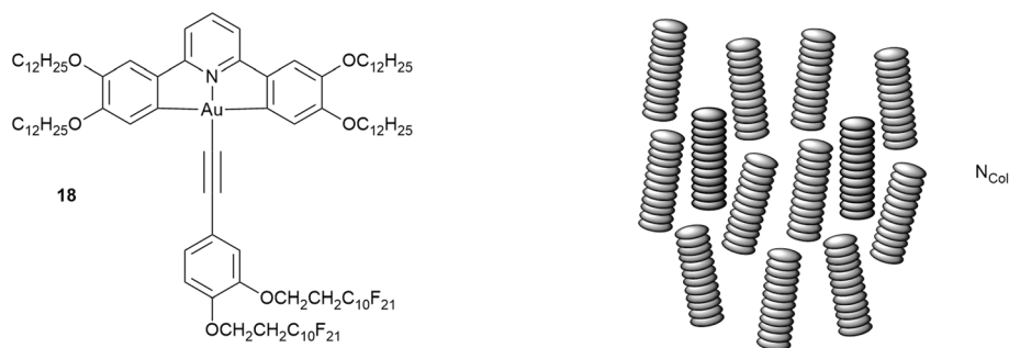
Fig. 26 Structure and LC phase behaviour of an amphiphilic gold complex and the organisation in the N_{\text{Col}} phase.
