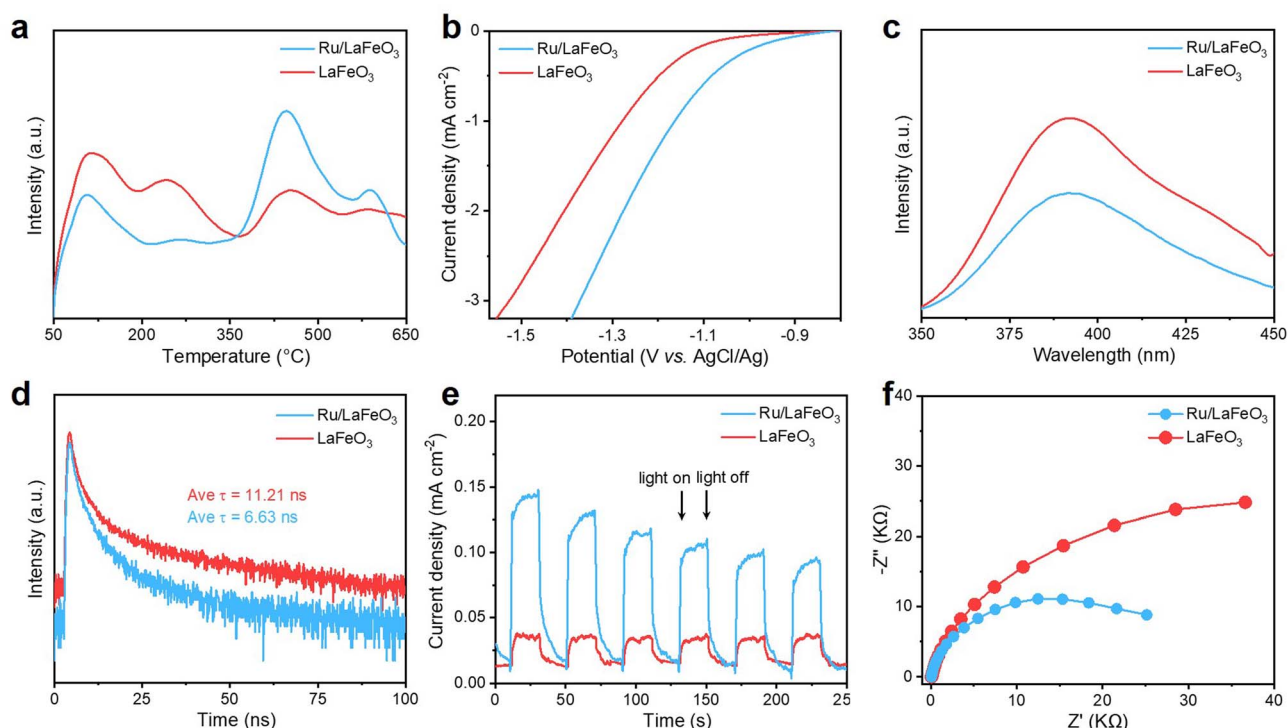
Fig. 3 (a) \text{CO}_2 -TPD, (b) LSV curves, (c) steady-state PL spectra, (d) TRPL spectra, (e) transient photocurrent responses, and (f) EIS Nyquist plots of \text{LaFeO}_3 and \text{Ru/LaFeO}_3 .
