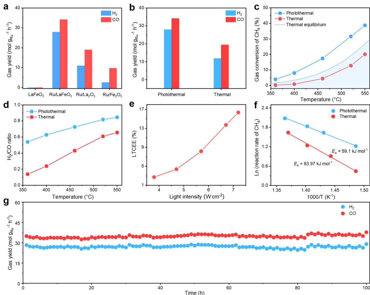
Fig. 2 (a) DRM performances of different catalysts under light-driven conditions (catalyst: 80 mg; light intensity: 6.7 W cm -2 ; feedstocks: CO 2 /CH 4 /He = 47/47/6, GHSV = 22.5 L g -1 h -1 ). (b) DRM activities of Ru/LaFeO 3 under photothermal and thermal conditions. (c) CH 4 conversion under photothermal and thermal conditions at different temperatures. (d) H 2 /CO ratios of DRM at different temperatures powered by pure light irradiation and external heating. (e) LTCEEs of Ru/LaFeO 3 under different incident intensities. (f) Arrhenius plots of CH 4 in photothermocatalysis and thermocatalysis by Ru/LaFeO 3 . (g) Stability test of Ru/LaFeO 3 in light-driven DRM.
