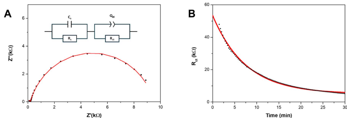
Fig. 2 Fitting EIS spectra to the equivalent circuit enables the quantification of the charge transfer resistance over time, giving insight into the kinetic rates of Au 25 deligation. (A) One representative EIS spectra (cycle 70) (black points), is fitted to the inset equivalent circuit (red line). (B) Equivalent circuit element R_{ct} (charge-transfer resistance to HER) vs. time (black points) is fitted to an exponential decay function (red line) to obtain a rate constant k_{delig} = 0.00222 \text{ s}^{-1} , R^2 = 0.9965 .
