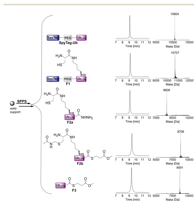
Fig. 3 Synthesis of SpyTag-Ub and the required building blocks for the preparation of the SpyTag-Ub variants using SPPS. Calculated masses: SpyTag-Ub: 10 606 Da, F1 : 10 709 Da, F2a : 8606 Da, F2b : 8706 Da, F3 : 8591 Da.
