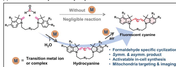
(b) This work: In-cell synthesis of cyclocyanines
