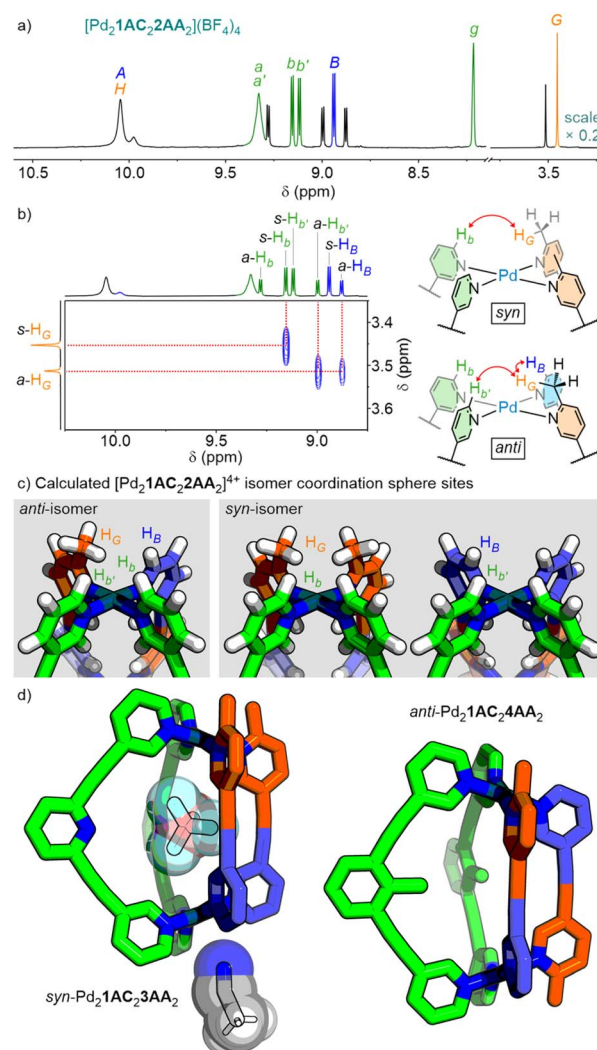
Fig. 4 (a) Partial ^1\text{H} NMR spectrum (600 MHz, \text{CD}_3\text{CN} , 298 K), with major \text{syn} -isomer peaks labelled, of [\text{Pd}_21\text{AC}_22\text{AA}_2](\text{BF}_4)_4 . (b) Partial NOESY spectrum (600 MHz, \text{CD}_3\text{CN} , 298 K) of [\text{Pd}_21\text{AC}_22\text{AA}_2](\text{BF}_4)_4 with key peaks used to identify the \text{syn} - ( s ) and \text{anti} -isomers ( a ). (c) Visualisation of the coordination sphere sites of \text{anti} - and \text{syn} - \text{Pd}_21\text{AC}_22\text{AA}_2 cage isomers from geometry-optimised models (GFN2-xTB). (d) SCXRD structures of \text{syn} - [\text{Pd}_21\text{AC}_23\text{AA}_2]^{4+} , showing endohedral \text{BF}_4^- counterion and exohedral \text{CH}_3\text{CN} solvent molecule interacting with the cage, and \text{anti} - [\text{Pd}_21\text{AC}_24\text{AA}_2]^{4+} .
