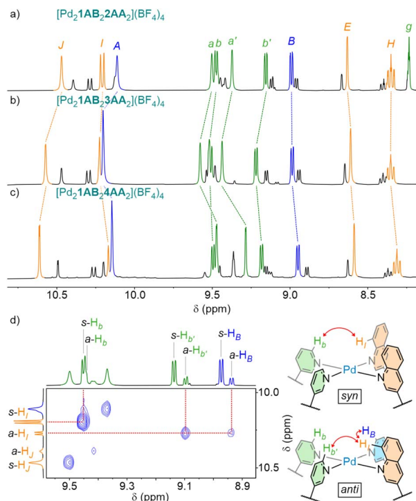
Fig. 3 Partial ^1\text{H} NMR spectra (400 MHz, \text{CD}_3\text{CN} , 298 K), with major \text{syn} -isomer peaks labelled, of (a) [\text{Pd}_21\text{AB}_22\text{AA}_2](\text{BF}_4)_4 , (b) [\text{Pd}_21\text{AB}_23\text{AA}_2](\text{BF}_4)_4 , and (c) [\text{Pd}_21\text{AB}_24\text{AA}_2](\text{BF}_4)_4 . (d) Partial NOESY spectrum (600 MHz, \text{CD}_3\text{CN} , 298 K) of [\text{Pd}_21\text{AB}_22\text{AA}_2](\text{BF}_4)_4 with key peaks used to identify the \text{syn} - ( s ) and \text{anti} -isomers ( a ).
