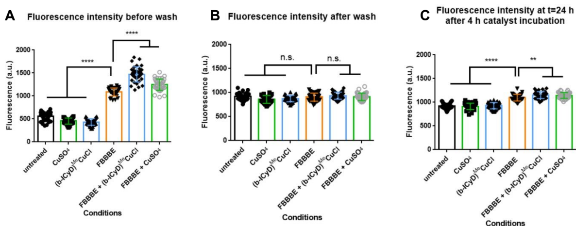
Figure 4. Bar charts detailing the fluorescence intensity of every tested condition for measurements after 2 h (Top) or 4 h (Bottom) incubation of the catalyst, before (A) and after (B) wash and at t = 24 h after the wash (C).
