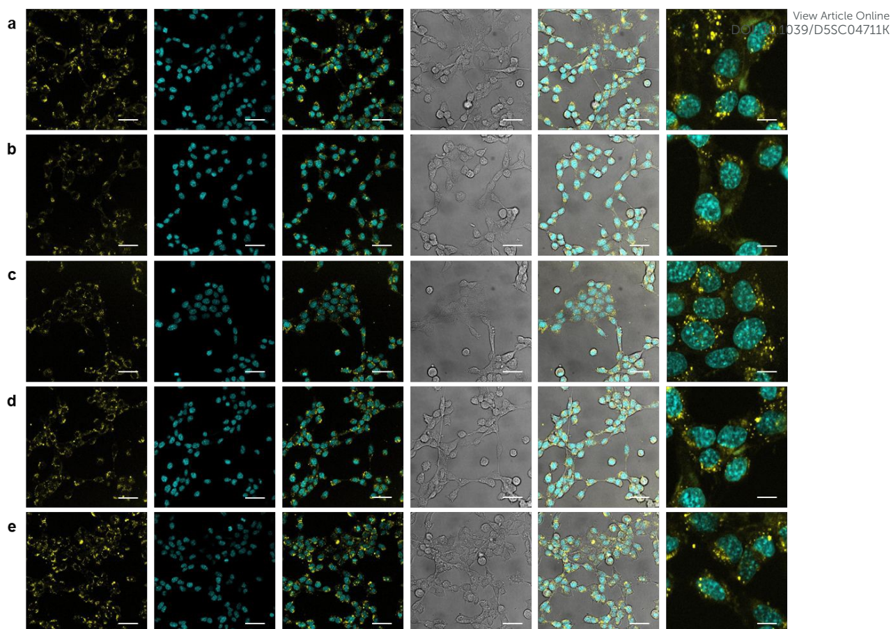
Figure 5. Intracellular fluorescence of fluorescein of CT26 cells treated only with FBBBE (a) or with FBBBE and 2 for 2 or 4 h (b and c, respectively), or with FBBBE and then with \text{CuSO}_4 for 2 or 4 h (d and e, respectively) by confocal microscopy. Cells were imaged live following incubation with FBBBE (yellow), Cu(I) compounds (not fluorescent), and then with Hoechst 33342 (cyan). In each line, the first panel (from left to right) is the fluorescein signal (yellow), the second panel is the nuclei image (cyan), the third panel is the merge of fluorescent channels, the fourth is the bright field image, the fifth is the merge of all the channels, and the sixth is a zoom of the merge of fluorescent channels. Scale bars are 40 \mu\text{m} for the non-zoomed images and 10 \mu\text{m} for the zoomed images.
