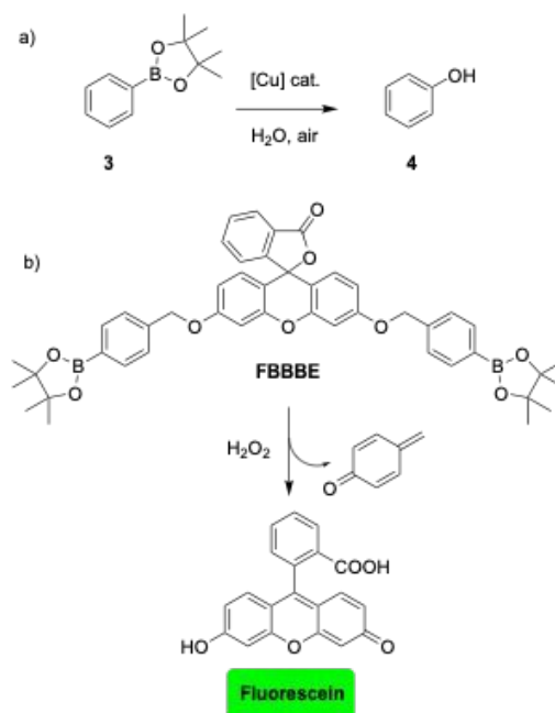
Figure 2. A) Copper-catalysed ipso -hydroxylation deborylation reaction; B) Principle of the self-immolative linker used in FBBBE profluorophore. FBBBE = Fluorescein bis(benzyl boronic ester).
