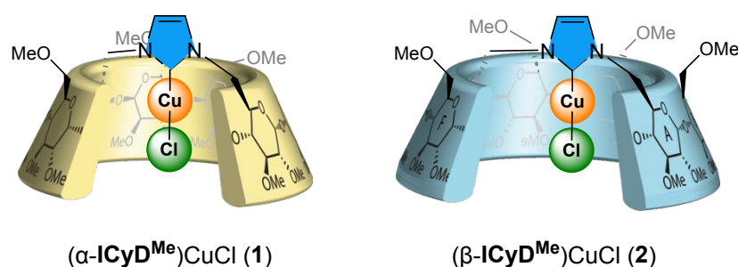
Figure 1. Water-soluble CD-NHC–copper(I) complexes [(α- ICyD Me )CuCl] ( 1 ) and [(β- ICyD Me )CuCl] ( 2 ) based on permethylated cyclodextrins, used in this study.
