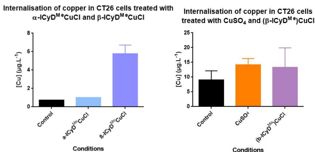
Figure 3. Internalisation of copper in cells treated A) (left) with [(\alpha\text{-ICyD}^{\text{Me}})\text{CuCl}] ( 1 ) and [(\beta\text{-ICyD}^{\text{Me}})\text{CuCl}] ( 2 ) compared to non-treated cells for 48 h; B) (right) with [(\beta\text{-ICyD}^{\text{Me}})\text{CuCl}] ( 2 ) or \text{CuSO}_4 compared to non-treated cells for 4 h.
