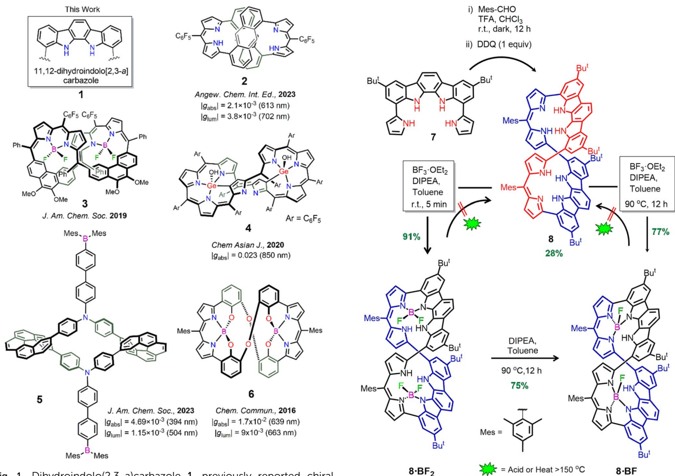
Scheme 1 Synthesis of macrocycle 8, bis- \text{BF}_2 complex 8 \cdot \text{BF}_2 , and bis-BF complex 8 \cdot \text{BF} . \text{Bu}^t = \text{tert-butyl} , TFA = trifluoroacetic acid, DDQ = 2,3-dichloro-5,6-dicyano-1,4-benzoquinone, DIPEA = diisopropylethylamine.
