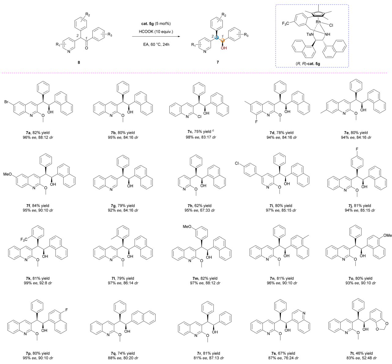
Scheme 2 Substrate scope of the DKR-ATH. a,b a Reaction conditions: the reactions were carried out with a catalyst/substrate (0.1 mmol) ratio of 1 : 20 in 1.0 mL of EA, HCOOK (10 equiv.) at 60 °C for 24 h; b all yields were of isolated products; dr values were determined via 1 H NMR analysis of the reaction mixtures; ee values were determined via HPLC analysis on a chiral stationary phase; c 50 °C, 48 h.
