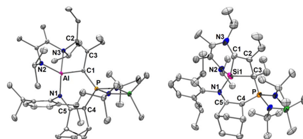
Fig. 4 Molecular structures of 5 (left) and 6 (right). Thermal ellipsoids represent 30% probability. H and disordered atoms are omitted for clarity. Selected bond lengths [Å] and angles [°]: 5: Al–N1 1.886(2), Al–N2 1.850(2), Al–N3 2.026(2), Al–C1 1.895(2), C1–C3 1.463(2), C3–C2 1.361(3), C2–N3 1.507(2), C1–P 1.670(2), N3–Al–C1 90.96(7), N3–Al–N2 86.66(6), N1–Al–C1 108.23(7), N1–Al–N2 120.12(7), Al–C1–C3 104.68(12), Al–C1–P 122.76(10), P–C1–C3 131.03(13). 6: C1–N3 1.398(9), C1–Al 1.849(8), Al–N2 1.821(7), Al–C3 2.145(8), C3–C2 1.534(10), C2–C1 1.400(10), C3–P 1.824(8), N1–Al 1.865(6), Al–C3–C2 82.6(4), C3–C2–C1 106.5(7), C2–C1–N3 135.2(8), C2–C1–Al 98.0(5), C1–Al–C3 71.7(3).
