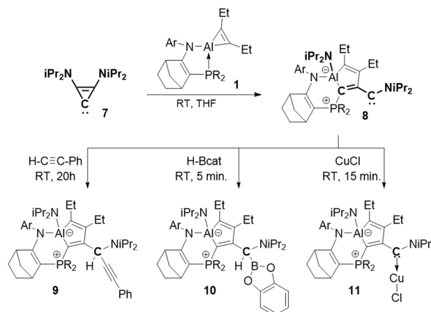
Scheme 2 The reaction of 1 with stable cyclopropenylidene 7 and reactions of (amino)carbene 8 .
