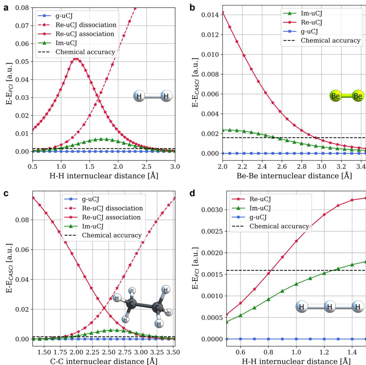
Fig. 1 Errors in energies for variational single reference calculations with g-uCJ, Re-uCJ and Im-uCJ ansätze relative to FCI or CASI energies for (a) H 2 , (b) Be 2 (2e,2o), (c) C 2 H 6 (2e,2o), and (d) linear H 3 + . The STO-3G basis set was used for all molecules. The horizontal black dashed line corresponds to chemical accuracy ( \sim 1 kcal mol ^{-1} , equivalent to 1.6 \times 10^{-3} a.u.). The RHF state was used as a reference state for all systems. The curves denoted by 'association' or 'dissociation' differ in how the initial guesses for the K and J matrices were obtained. For the association curves, the optimized parameters from the prior step were used as the initial guess at the next step as the bond distance was gradually decreased. In contrast, for the dissociation curves, the bond distance was gradually increased.
