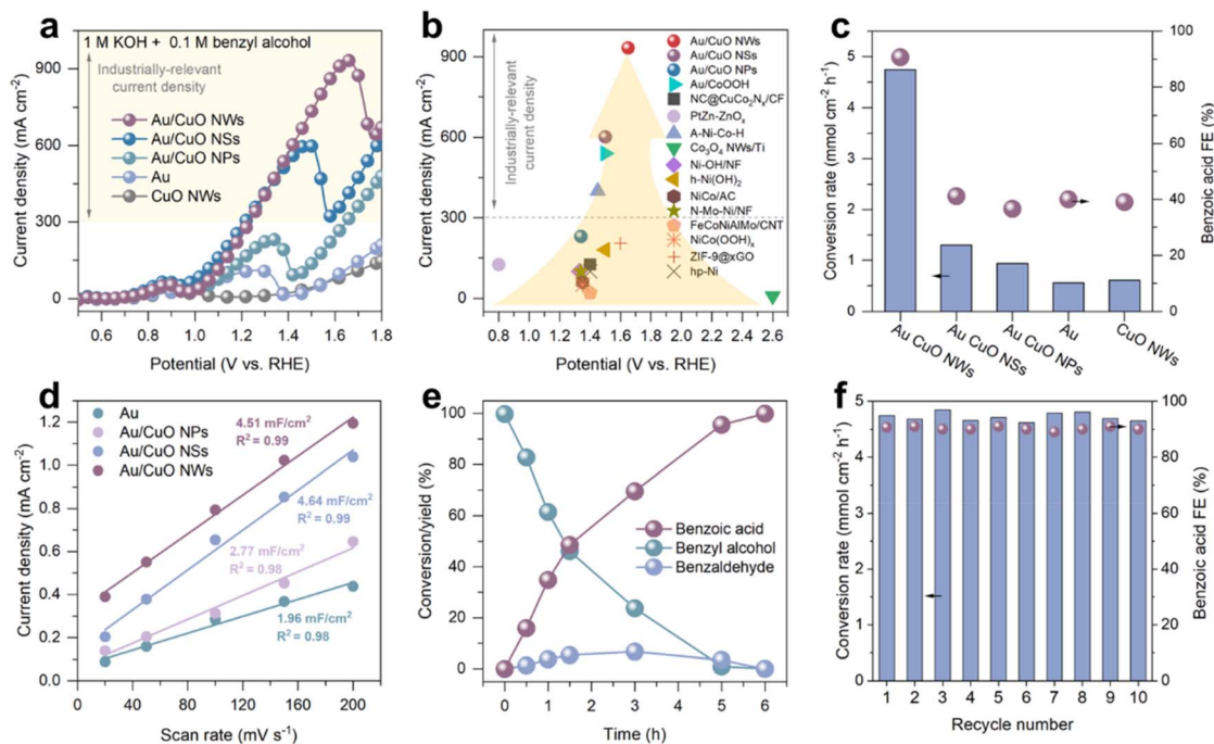
Fig. 2 (a) LSV curves of benzyl alcohol electrooxidation at scan rate of 10 mV s -1 in 1 M KOH with 0.1 M benzyl alcohol over different catalysts. (b) Current densities of benzyl alcohol electrooxidation in the literature and in this work. (c) Conversion rate of benzyl alcohol and the corresponding FE of benzoic acid over different catalysts. (d) The charging currents measured plotted as a function of scan rate. (e) Kinetic curves for benzyl alcohol oxidation over Au/CuO NWs at 1.5 V vs. RHE. (f) Stability test of Au/CuO NWs for benzyl alcohol oxidation in batch reaction (10 batches, 10 h).
