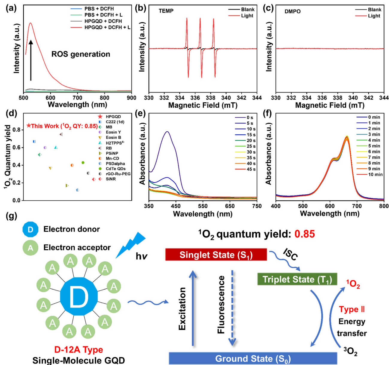
Fig. 3 Excellent ROS generation ability of HPGQD. (a) ROS generation test. DCFH ( 1 \times 10^{-7} mol L -1 ) was used to detect ROS generation of HPGQD with/without light irradiation (460 nm, 20 mW cm -2 , 30 s). (b) ESR-based ROS species test utilizing TEMP as an indicator probe for singlet oxygen ( 1 O 2 ). The ESR signal indicative of 1 O 2 was obtained after exposing HPGQD solution to a xenon lamp (300 W) for 30 s, with TEMP serving as the trapping agent. (c) ESR-based ROS species test utilizing DMPO as an indicator probe for • OH. The ESR signal indicative of • OH was obtained after exposing HPGQD solution to a xenon lamp (300 W) for 30 s, with DMPO serving as the trapping agent. (d) Comparative analysis of 1 O 2 quantum yield of previous works. (e) UV-vis-based ROS species and generation efficiency test using DPBF as a probe for 1 O 2 . HPGQD (0.83 μmol L -1 , 3 mL) was irradiated at different times and 1 O 2 was detected using DPBF (0.25 mg mL -1 , 200 μL). (f) UV-vis-based ROS species and generation efficiency test using MB as a probe for • OH. HPGQD (0.83 μmol L -1 , 3 mL) was irradiated at different times and • OH was detected using MB (300 μmol L -1 , 1 mL). (g) Mechanism of generating 1 O 2 by HPGQD.
