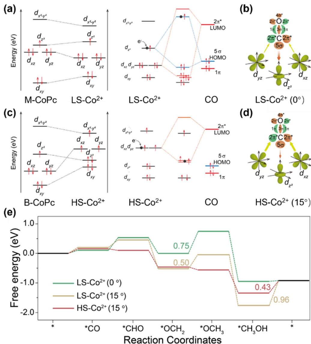
Fig. 5 (a) and (c) 3d orbital diagrams of M-CoPc and B-CoPc after heat treatments and the corresponding illustration of interactions with CO molecular frontier orbitals ( 5\sigma and 2\pi^* ). Black dots represent the electrons from electrodes under cathodic bias. (b) and (d) Schematic of \sigma and \pi -donation bonds between CO and 3d orbitals of LS-Co 2+ and HS-Co 2+ . (e) Free energy diagram of the CORR over LS-Co 2+ and HS-Co 2+ . 74 Reproduced from ref. 74 with permission from Springer Nature, copyright 2023.
