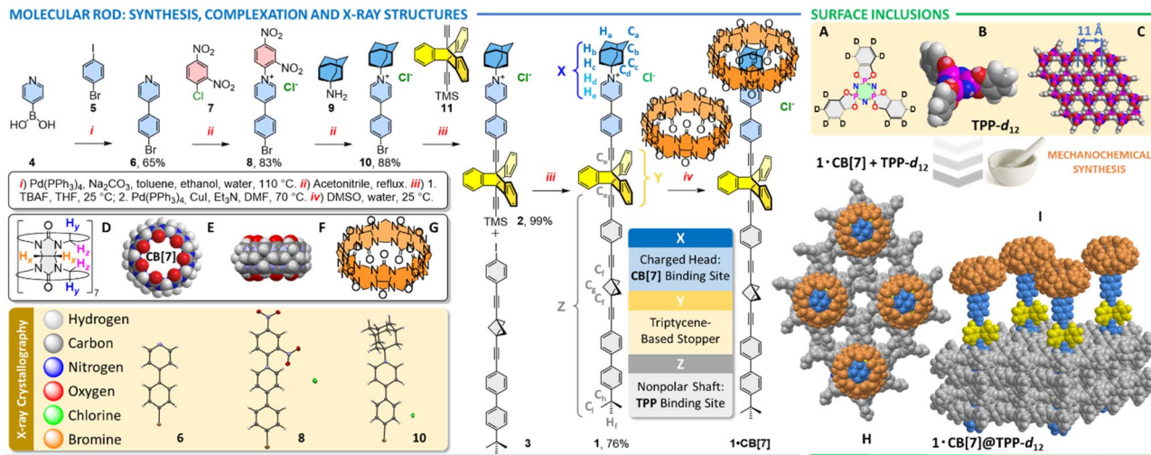
Fig. 1 Synthesis of molecular rod 1 and its reaction with CB[7] leading to supramolecular complex 1 · CB[7] . The structure of the TPP- d 12 molecule (A), the corresponding space-filling model (B) and a top view of a small fragment of hexagonal TPP (C). CB[7] : a schematic representation (D), top (E) and side (F) view on a space-filling model, and a chemical structure (G). Idealized graphical visualization of surface inclusion 1 · CB[7] @ TPP- d 12 : top (H) and side (I) view on a space-filling model. ORTEP representation of intermediates 6 , 8 , and 10 (thermal ellipsoids shown on 30% probability level).
