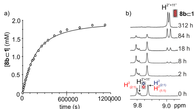
Fig. 5 (a) Changes in the concentration of 8b ⋅ 1 over time determined using the integral areas of protons H 2' and H 11' . The solid line represents the fit of the experimental kinetic data to the theoretical model using COPASI V4.25. (b) Selected region of the 1 H NMR spectra of the kinetic study of the formation of 8b ⋅ 1 starting from a 1 : 1 : 1 mixture of 2b , 4 , and octa-imine cage 1 . The selected region corresponds to the area in the 1 H NMR spectrum where the pyrrole NH protons resonate.
