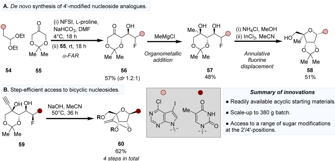
Fig. 6 De novo synthesis of nucleosides starting from acyclic precursors. (A) Preparation of 4'-modified and (B) bicyclic nucleoside analogues.
