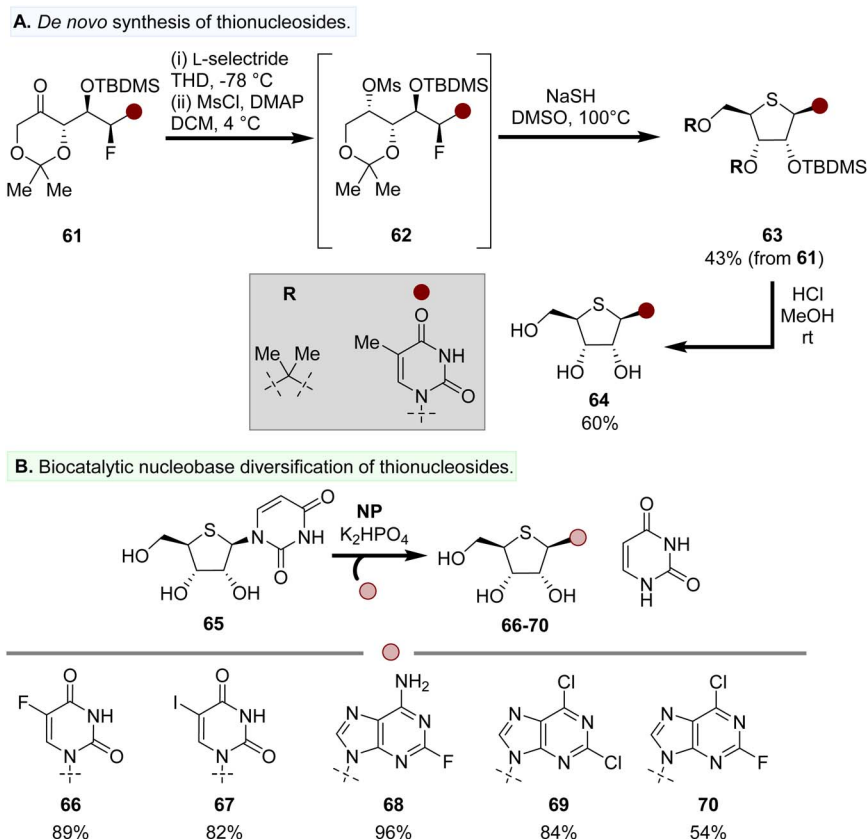
Fig. 7 Preparation of thionucleosides by (A) de novo synthesis and (B) a biocatalytic base swapping approach.
