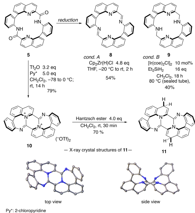
Scheme 4 Derivatization from cyclic diamide 5 .
