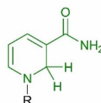
1,2-NAD(P)H (enzymatically inactive)
