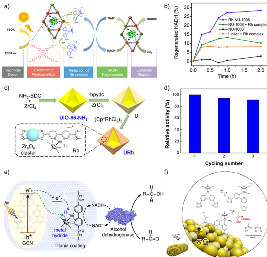
Fig. 7 Integration of Rh-M with various light-harvesting components. (a) Schematic showing the photo-enzymatic conversion of CO 2 to formic acid using Rh-M integrated and FDH encapsulated NU-1006 MOF. (b) NADH regeneration by Rh-M integrated NU-1006 MOF compared with the physical mixture of NU-1006 and freely diffusing Rh-M shows an enhanced charge transfer rate. Adapted with permission from ref. 86. Copyright 2020 American Chemical Society. (c) Schematic representation of core-shell MOF for integration of Rh-M with the light-harvesting component. (d) Plot showing the 1,4-NADH regeneration activity for multiple cycles, which confirms negligible loss of Rh-M from the surface of core-shell MOF. Adapted with permission from ref. 78. Copyright 2020 American Chemical Society. (e) Schematics of the photo-enzymatic system for methanol production with Rh-M embedded in a porous TiO 2 over graphitic carbon nitride (GCN) to spatially separate it from the ADH enzyme. Such a strategy prevented aggregation-induced deactivation of the ADH enzyme. Adapted with permission from ref. 85. Copyright 2021 American Chemical Society. (f) Schematics showing the photoregeneration of 1,4-NADH with Rh-M modified CdS nanorods. The carboxylate groups of bipyridine moiety in Rh-M coordinate with surface Cd 2+ and displace parent thiolate ligands. Adapted with permission from ref. 88. Copyright 2024 American Chemical Society.
