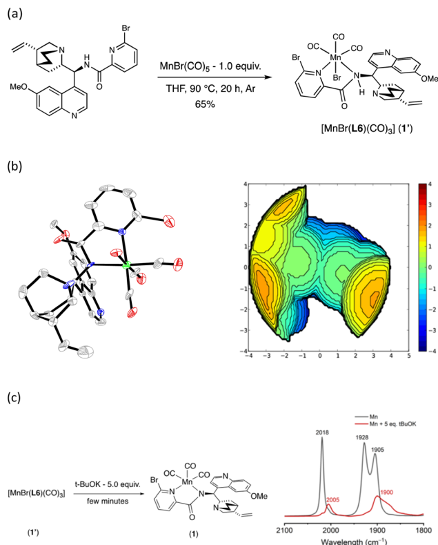
Scheme 2 (a) Synthesis of [\text{Mn}(\text{i})\text{Br}(\text{L6})(\text{CO})_3] ( 1' ). (b) Solid-state structure of complex ( 1' ) (hydrogen omitted for clarity) and steric map of the isolated \text{Mn}(\text{i}) cinchona complex. Total % V_{\text{bur}} by the ligand is 43.5%. % V_{\text{bur}} by each quadrant are 44.7% (SW), 55.1% (NW), 25.4% (NE), 48.9% (SE). (c) IR spectra of active [\text{Mn}] complex 1' (black) and the in situ -generated imido complex 1 (red) recorded in THF at 25 °C.
