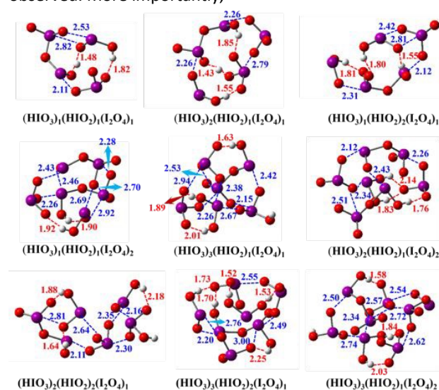
Figure 2. Global minimum configurations of the (HIO_3)_x(HIO_2)_y(I_2O_4)_z ( x = 1-3 , y + z = 2-3 ) clusters calculated at the DLPNO-CCSD(T)/aug-cc-pVTZ(-PP)//M06-2X/aug-cc-pVTZ(-PP) level of theory. The red balls represent oxygen atoms, purple ones are for iodine atoms, and white ones are for hydrogen atoms. The red dashed lines represent HBs, and the blue dashed lines represent XBs. The red and blue numbers indicate the bond lengths of HBs and XBs, respectively. The bond lengths are given in Å.
