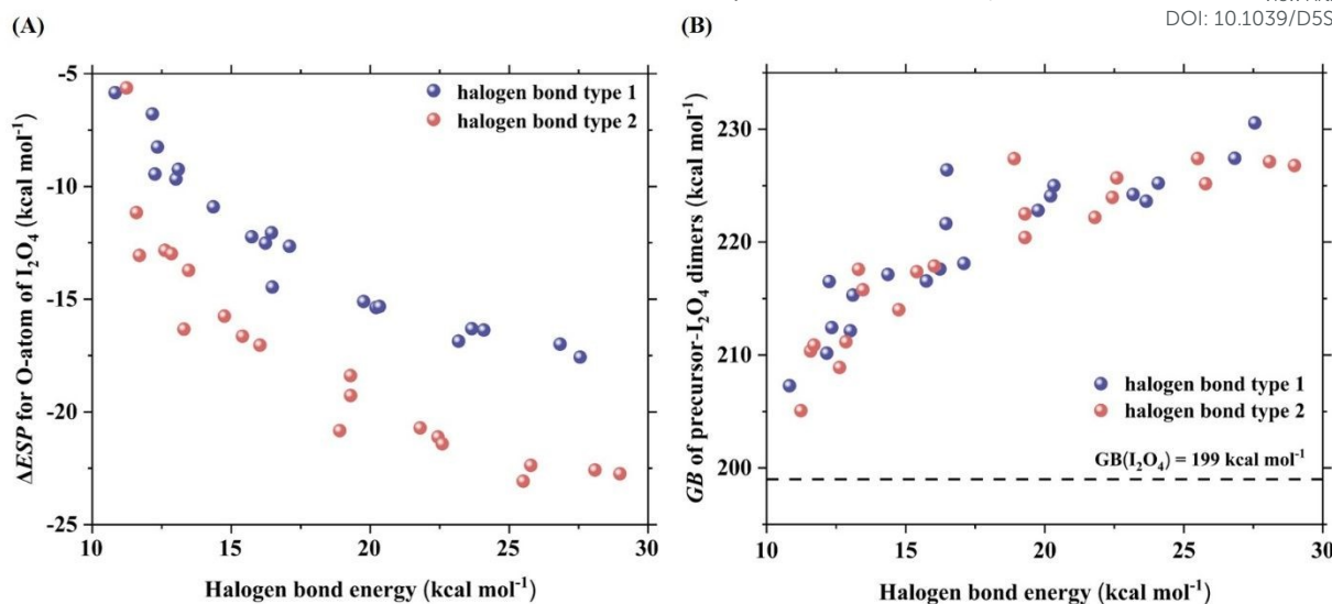
Figure 3. Change in electrostatic potential ( \Delta\text{ESP} ) values ( \text{kcal mol}^{-1} ) for the O atom as a basic site of \text{I}_2\text{O}_4 (A) and the gas basicity (GB) ( \text{kcal mol}^{-1} ) of precursor- \text{I}_2\text{O}_4 dimers (B) as a function of the halogen bond energy ( \text{kcal mol}^{-1} ). The purple and red spheres represent two different types of XBs. O-atom 1 is the basic site of \text{I}_2\text{O}_4 when it forms XB type 1 with precursors. O-atom 2 is the basic site of \text{I}_2\text{O}_4 when it forms XB type 2 with precursors.
