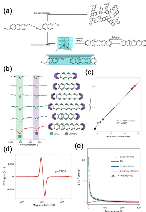
Fig. 28 (a) Schematic of polyacene synthesis using an MOF. (b) FTIR spectra of tetracene, pentacene, hexacene, heptacene and polyacenes. (c) The relative peak area of SOLO to QUATRO vibration modes ( A_{\text{SOLO}}/A_{\text{QUATRO}} ) plotted against the benzene ring number for the acene series. (d) ESR spectrum of polyacene. No hyperfine splitting was observed, suggesting the delocalization of spin density along the polymer chains. (e) Temperature dependence of the magnetic susceptibility \chi of polyacene. Reproduced with permission from ref. 101. Copyright 2023 Springer Nature.
