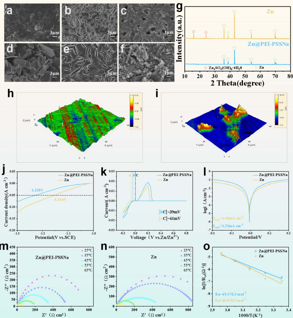
Fig. 3 SEM images of (a) Zn@PEI-PSSNa and (d) bare Zn after 50 cycles in a symmetric cell at 1 mA cm -2 and 1 mAh cm -2 . SEM images of (b) Zn@PEI-PSSNa and (e) bare Zn after 30 days of immersion in 2 M ZnSO 4 . Scanning electron microscopy images of (c) Zn@PEI-PSSNa and (f) bare Zn after 50 cycles in a Zn||Cu cell at a current density of 1 mA cm -2 and 1 mAh cm -2 . (g) Comparison of XRD images after 50 cycles at 1 mA cm -2 and 1 mAh cm -2 . HRCM images of (h) Zn@PEI-PSSNa and (i) bare Zn after 50 cycles at 1 mA cm -2 and 1 mAh cm -2 . (j) LSV testing of materials. (k) CV curve of the Zn||Cu cell. (l) Tafel curves for samples. Nyquist plots of (m) Zn@PEI-PSSNa and (n) bare Zn at different temperatures. (o) Arrhenius curve corresponding to the sample.
