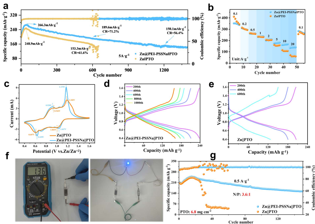
Fig. 5 (a) Comparative cycling performance of full batteries at a current density of 5 \text{ A g}^{-1} . (b) Multiplier performance test for full batteries. (c) CV curves for the full batteries at 1 \text{ mV s}^{-1} sweep speed. Charge–discharge curves of the full batteries using (d) Zn@PEI-PSSNa and (e) bare Zn anode. (f) Test photo of the small pouch-cell and (g) cycling performance of the pouch cell at a high mass loading of the cathode material.
