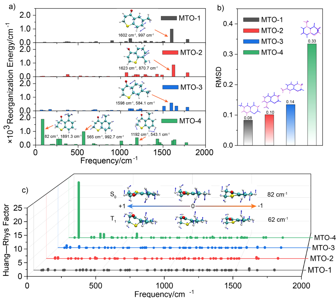
Fig. 4 (a) Calculated reorganization energies of the T_1 \rightarrow S_0 transition are plotted against the frequencies of MTOs. Representative high-intensity (>500 \text{cm}^{-1} ) vibration modes are shown as insets; (b) schematic distribution of RMSD T_0 \rightarrow S_0 values; (c) Huang-Rhys factors of MTOs from T_1 to S_0 . The insets show the most representative intramolecular vibration modes of MTO-4 in S_0 and T_1 states.
