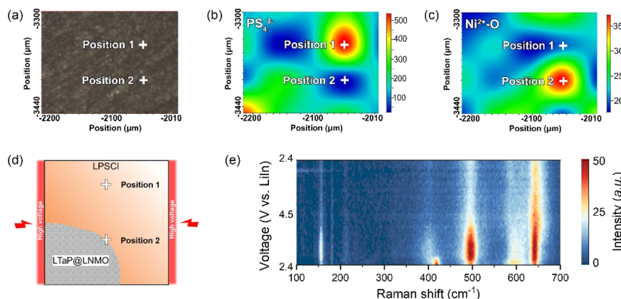
Fig. 3 (a) Micrograph of the in situ Raman surface scanning mode and selected points in the LTA@LNMO-LPSCI-VGCF|LPSCI|LiIn cell. (b and c) Distribution of the cathode and sulfide electrolyte, distinguished by observing the local content distribution of \text{PS}_4^{3-} ( 420\text{ cm}^{-1} ) and \text{Ni}^{2+}\text{-O} ( 490\text{ cm}^{-1} ) in the composite cathode, respectively. (d) Schematic diagram of position 1 and position 2 studied in the in situ Raman experiments. (e) The in situ Raman spectra of the LTA@LNMO-LPSCI-VGCF composite cathode at position 2 from a two-dimensional view.
