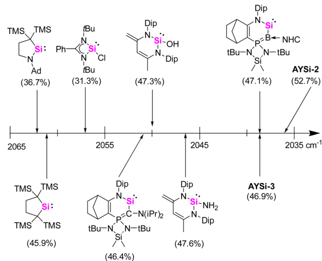
Fig. 4 Comparison of the TEP values for various silylenes determined by asymmetric CO stretching frequency of \text{LNi(CO)}_3 in toluene at room temperature. 26,31 % \nu_{\text{bur}} is given in parentheses.
