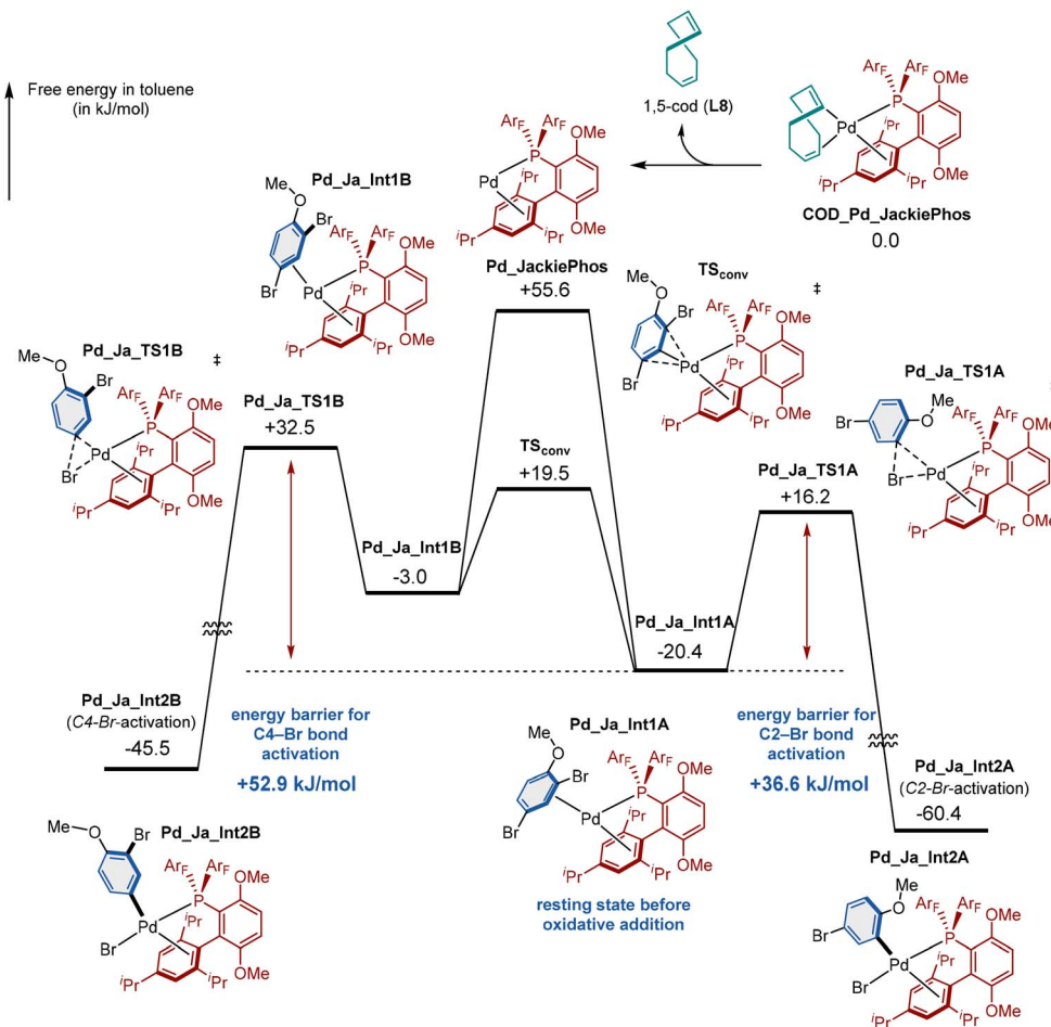
Fig. 1 DFT calculations for the oxidative-addition step of 1a to Pd_JackiePhos. Relative Gibbs energy values (in kJ mol -1 ) were calculated at the B3LYP-D3/6-311G(d,p)//B3LYP-D3/6-311G(d,p) level (SDD basis sets used for Br and Pd) using the implicit IEF-PCM solvation model (solvent = toluene).
