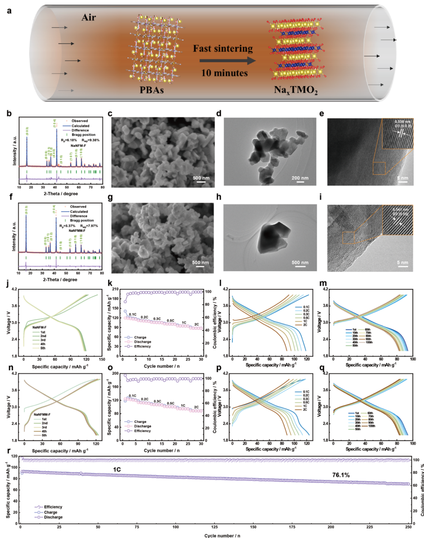
Fig. 4 (a) Schematic diagram of the transformation process from PBAs to layered oxides. (b) Powder XRD result with Rietveld refinement of NaFM-F. (c) SEM, (d) TEM, and (e) HRTEM images of NaFM-F. (f) Powder XRD result with Rietveld refinement of NaFMM-F. (g) SEM image of NaFMM-F. (h) TEM and (i) HRTEM images of NaFMM-F. Electrochemical performance of the electrode within the potential window of 2–4 V: GCD curves at 0.1 C for (j) NaFM-F and (n) NaFMM-F. Rate performance of (k) NaFM-F and (o) NaFMM-F. GCD curves at different rates of (l) NaFM-F and (p) NaFMM-F. GCD curves at different cycles of (m) NaFM-F and (q) NaFMM-F. (r) Cycling performance of NaFMM-F.
