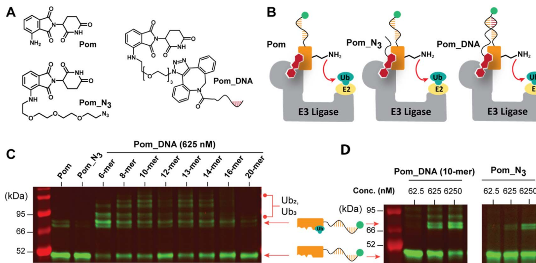
Fig. 3 (A) Structures of glutarimide derivatives and the corresponding DNA-linked version after bioconjugation. (B) In vitro ubiquitin transfer of Pom, Pom_N3, and Pom_DNA were tested and compared. (C) DNA templated Ub-transfer to IKZF1a with Pom, Pom-N3 and varying lengths of Pom_DNA (detailed conditions: ESI Section 5†). (D) The in vitro reconstituted CRL4 CRBN E3 ligase targeting the IKZF1a, using Pom_DNA (10-mer) as the molecular glue (left) or Pom_N3 (right) at different concentrations (see ESI Section 7† for additional experiments on DNA length dependence, effect of linker and DNA positioning as well as a panel of controls for the in vitro Ub-transfer).
