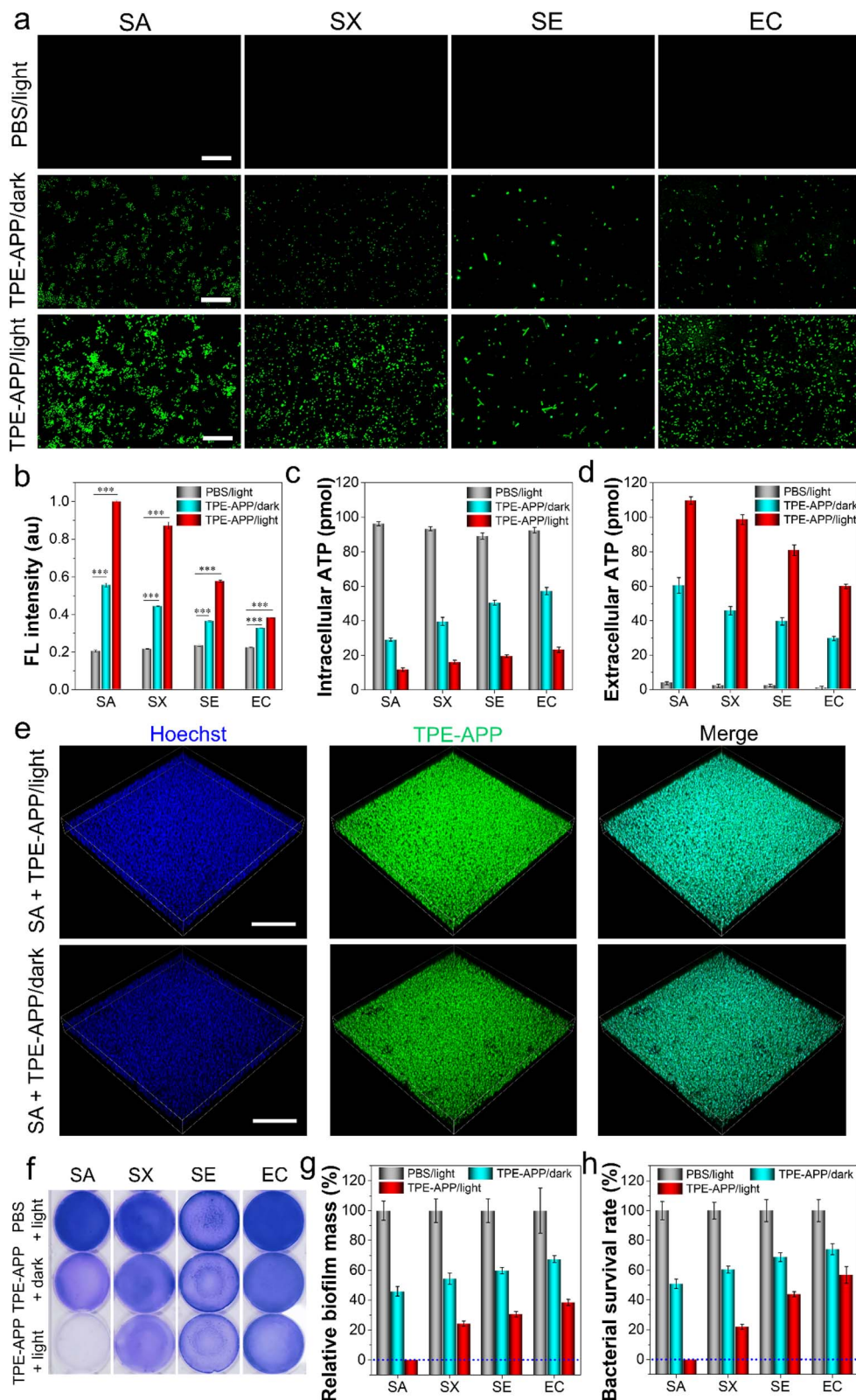
Fig. 4 Bacterial killing by TPE-APP probes through ROS caused cell membrane damage. (a) ROS generation in SA, SX, SE and EC ( 5 \times 10^7 CFU \text{mL}^{-1} ) after treatment with TPE-APP ( 120 \mu\text{M} ) for 2 h, followed by either dark conditions or white light irradiation ( 30 \text{ min} , 5 \text{ mW cm}^{-2} ), measured using DCFH-DA ( 10 \mu\text{M} ) as an indicator. Scale bar: 10 \mu\text{m} . (b) Membrane potential changes in SA, SX, SE and EC treated with TPE-APP probes under different conditions. ***P < 0.001 . (c and d) Extracellular and intracellular ATP levels of different bacteria treated with 120 \mu\text{M} TPE-APP for 2 h, followed by either dark conditions or white light irradiation ( 40 \text{ min} , 5 \text{ mW cm}^{-2} ). (e) Biofilm imaging after treatment with TPE-APP under dark conditions or white light irradiation ( 5 \text{ mW cm}^{-2} ) for 60 min. Blue color represents Hoechst for nucleus staining ( \lambda_{\text{ex}} = 405 \text{ nm} , \lambda_{\text{em}} = 430\text{--}475 \text{ nm} ), and green color represents TPE-DMA ( \lambda_{\text{ex}} = 405 \text{ nm} , \lambda_{\text{em}} = 500\text{--}550 \text{ nm} ). Scale bar: 500 \mu\text{m} . (f) Crystal violet staining of biofilms formed by
