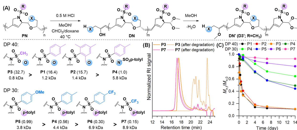
Fig. 4 (A) Degradation reaction pathway. Structures of polymers, normalized relative degradation rates (in parenthesis), and M n of the degraded product after 14 days. (B) SEC traces of P3 and P7 degradation under 0.5 M HCl acidic conditions. (C) Plots of degradation versus time for P1–P7 . M n,0 refers to the initial molecular weight and M n,t refers to the molecular weight at time t (days). The ratio M n,t / M n,0 was normalized to 1 for comparison.
