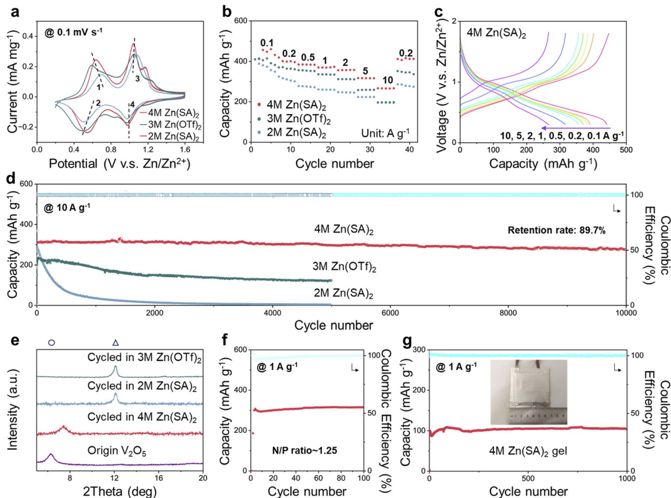
Fig. 5 Performance of ZMB cells. (a) CV curves of the V_2O_5/Zn cells with Zn(SA)_2 and Zn(OTf)_2 electrolytes at 0.1 \text{ mV s}^{-1} , in which two redox pairs, e.g., 0.63/0.54 and 1.04/0.97 in 4 M Zn(SA)_2 , can be attributed to H^+/Zn^{2+} insertion/desertion in mixed valence state V_2O_5 . 22,70 (b) Rate performance of the full cells comparing the Zn(SA)_2 and Zn(OTf)_2 electrolytes. (c) Galvanostatic charge–discharge curves of the cell with 4 M Zn(SA)_2 at a series of current densities from 0.1 to 10 \text{ A g}^{-1} . (d) Long-term cycling of the full cells with zinc aqueous electrolytes at 10 \text{ A g}^{-1} . (e) Ex situ XRD patterns of the cycled V_2O_5 cathodes in different electrolytes at 1 \text{ A g}^{-1} , which show the presence of crystalline phases of V_2O_5 (○) and ZVO (△). (f) Cycling of the full cell at 1 \text{ A g}^{-1} with an N/P ratio of \sim 1.25 . (g) Pouch cell with the gel electrolyte cycled at 1 \text{ A g}^{-1} .
