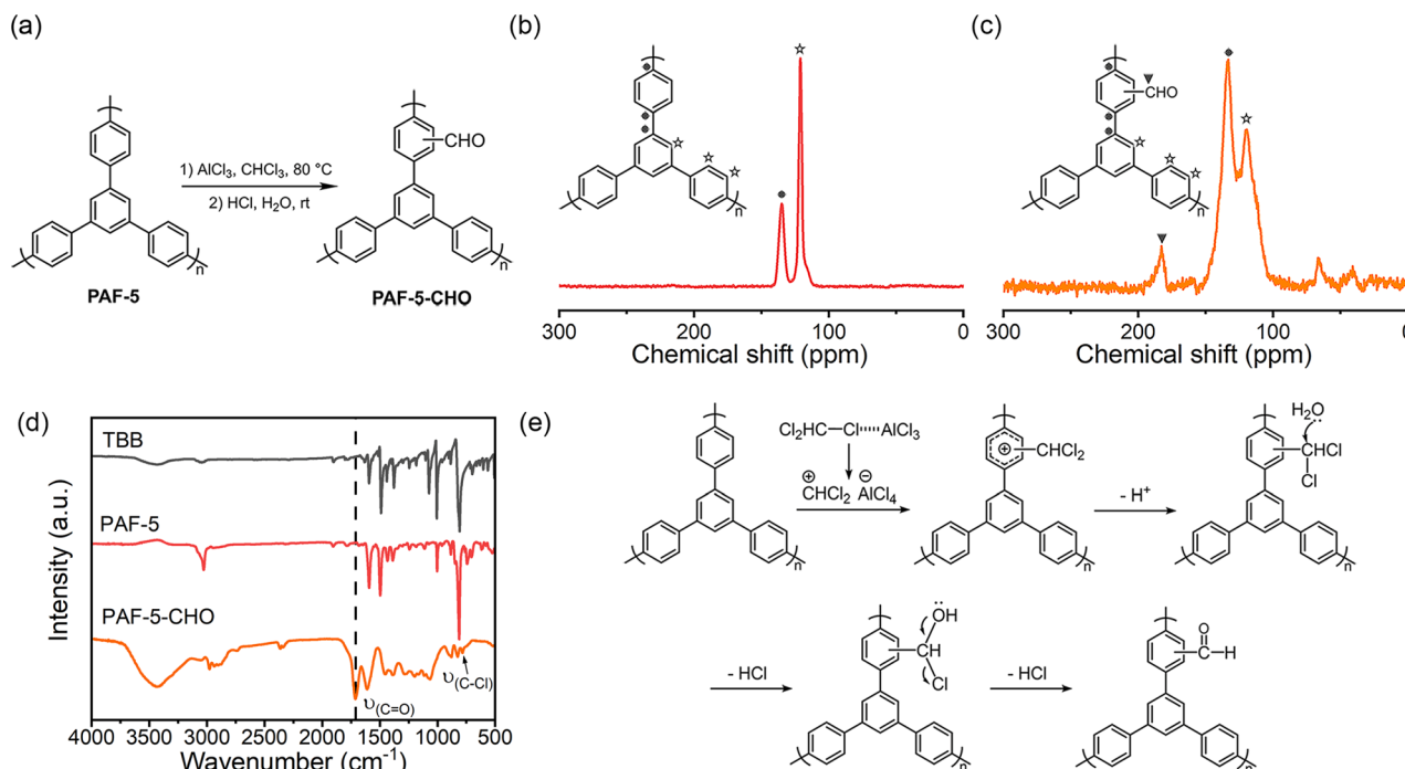
Fig. 1 (a) The synthesis of PAF-5-CHO; (b) 13 C CP/MAS NMR spectrum of PAF-5; (c) 13 C CP/MAS NMR spectrum of PAF-5-CHO. (d) FTIR spectra of PAF-5-CHO, PAF-5, and TBB (1,3,5-tris(4-bromophenyl) benzene); (e) the formation mechanism of –CHO groups.
