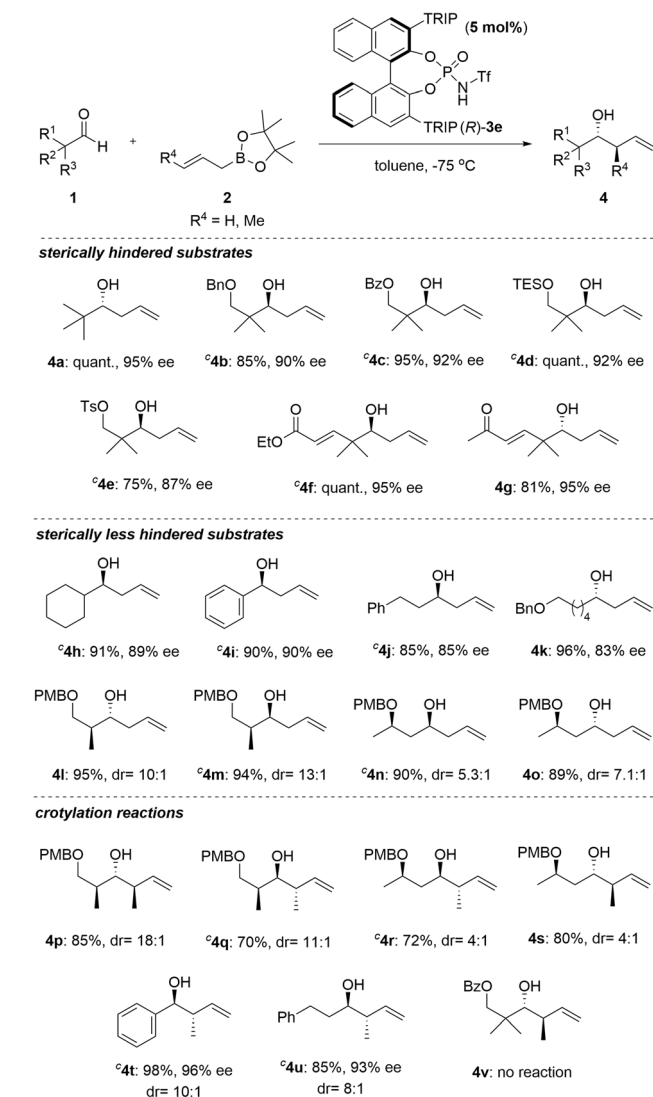
Scheme 4 a Unless otherwise specified, all reactions were carried out using 0.20 mmol of 1a , 0.24 mmol (1.2 eq.) of 2 , and 0.010 mmol (5 mol%) of catalyst. b Isolated yield. c ( S )- 3e was used instead of ( R )- 3e . TRIP = 2,4,6- t Pr 3 -C 6 H 2 . Chiral phosphoramidate-catalysed allylation and crotylation of aldehydes. a,b
