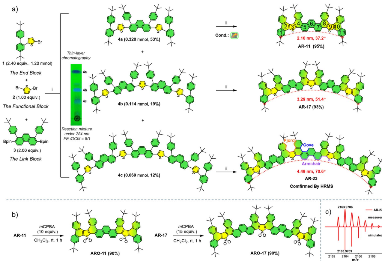
Scheme 1 The synthesis of thiophene-backbone arcuate GNRs. (a) (i) 1 (2.4 equiv.), 2 (1.0 equiv.), 3 (2.0 equiv.), Pd(PPh 3 ) 4 (0.5 equiv.), K 2 CO 3 (25 equiv.), 1,4-dioxane:H 2 O = 8:1: 90 °C, 36 h. Isolated yields were based on the amount of compound 1 . Thin-layer chromatography: TLC was run three times with the eluent system (PE/DCM = 8/1). (ii) DDQ (1.2 equiv. for each C–C bond), CF 3 SO 3 H, CH 2 Cl 2 , –10 °C, 1 h. DDQ: 2,3-dichloro-5,6-dicyano-1,4-benzoquinone. Electrochemical continuous flow conditions: a carbon anode, a Ni cathode, n Bu 4 NBF 4 (0.13 M), DCM/TFA, 4a (0.1 mmol), 1.65 V, 0.10 mL min –1 , rt. (b) Synthetic route of ARO-11 and ARO-17 . (c) High-resolution MALDI-TOF mass spectra of AR-23 .
