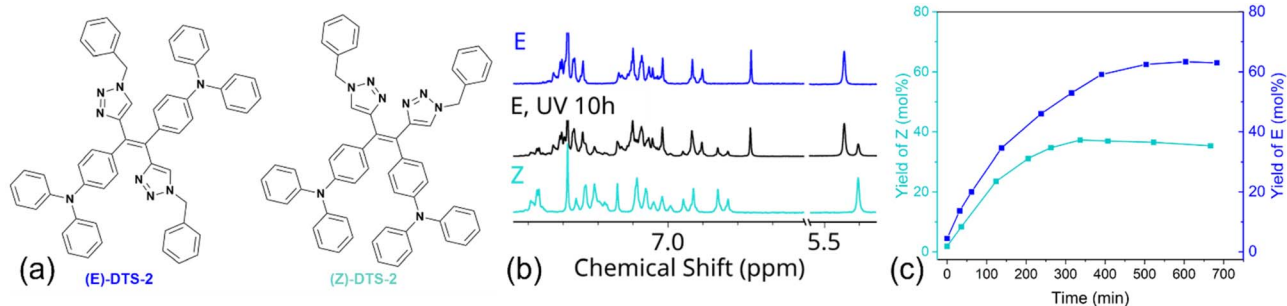
Fig. 5 (a) Structure of the isolated diastereoisomers of DTS-2 (b) partial 1 H NMR spectra of (E) -DTS-2 (blue), of irradiated (E) -DTS-2 (black) and (Z) -DTS-2 (cyan). (c) Isomerization yield of the initially pure (E) (blue) and (Z) (cyan) in CD 2 Cl 2 (10 −3 M) upon photoirradiation at 365 nm (4.7 mW cm −2 ) determined by NMR.
