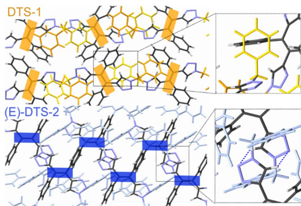
Fig. 3 Crystal structure of (E) -DTS-1 (top) and (E) -DTS-2 (bottom). Central double bonds are highlighted with a rectangle to show specific packing: herringbone (orange, (E) -DTS-1) and \beta -motif (blue, (E) -DTS-2). Zooms show specific intermolecular interactions: T-contacts in DTS-1 and triazole \pi -stacking in (E) -DTS-2.
