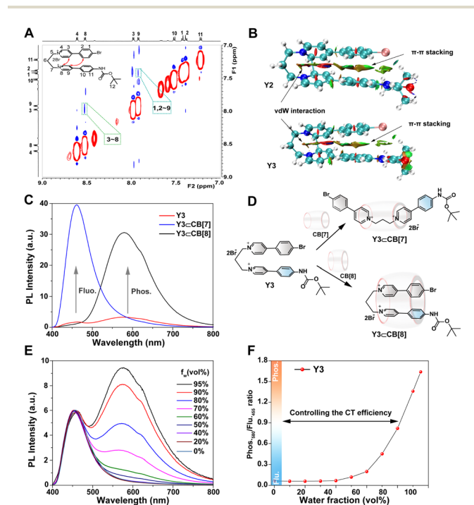
Fig. 4 Characterization of single-molecular luminescent properties. (A) Sectional 2D-ROESY-NMR spectrum of Y3 (1 mM in D 2 O and at 298 K). (B) IGMH isosurfaces and folded conformations of Y2 and Y3 . (C) PL spectra of adding equivalent amounts of CB[7] and CB[8] into the Y3 aqueous solution. (D) Schematic of the supramolecular regulation method for the Y3 molecular conformation variation. (E) Normalized PL spectra of Y3 solutions at various volume fractions of MeOH and water (from 0 to 100%, f_w ), the fluorescence intensity at 455 nm was unified. (F) Phosphorescence/fluorescence (phos. 580 /fluor. 455 ) intensity ratio as a function of water fraction f_w .
