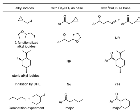
Fig. 4 Comparison of MIC catalyzed coupling reactions with \text{Cs}_2\text{CO}_3 and t BuOK.
