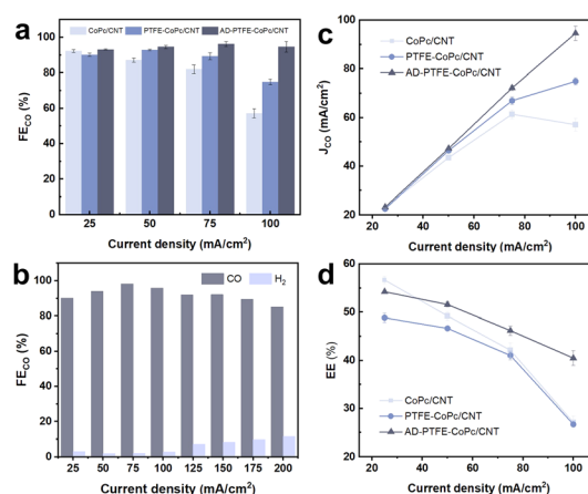
Fig. 5 (a) FE CO for CoPc/CNT, PTFE-CoPc/CNT, and AD-PTFE-CoPc/CNT at a series of applied currents in a MEA. (b) FE CO of AD-PTFE-CoPc/CNT in a wider range of series currents in the MEA. (c and d) J CO and EE of the CO 2 RR for CoPc/CNT, PTFE-CoPc/CNT, and AD-PTFE-CoPc/CNT.
