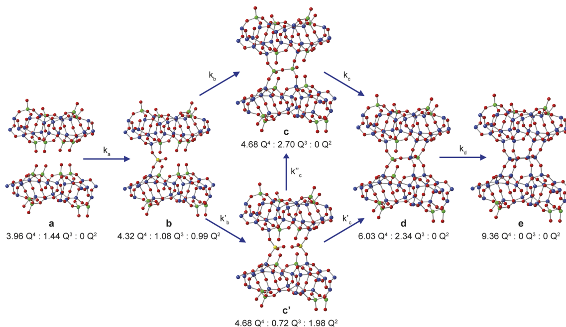
Fig. 5 Schematic showing the proposed mechanism of intercalation of \text{Si(OH)}_4 into the layers of IPC-1P. The ratios of NMR-active ^{29}\text{Si} \text{Q}^4 , \text{Q}^3 and \text{Q}^2 species for each of the structural models a , b , c , c' , d and e are given. Oxygen atoms are shown in red, and \text{Q}^2 , \text{Q}^3 and \text{Q}^4 Si atoms in yellow, green and blue, respectively.
