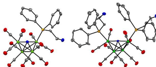
Fig. 1 Solid state structures of (left) 1^- in \text{Et}_4\text{N-1}\cdot\text{THF} , 18 and (right) 2^- in \text{PPN-2} . 19 Gray, blue, green, orange ellipsoids represent C, N, Fe, O and P atoms, respectively. Ellipsoids are shown at 50%; counter cations ( \text{Et}_4\text{N}^+ and \text{PPN}^+ ), solvates, and H atoms are omitted for clarity.
